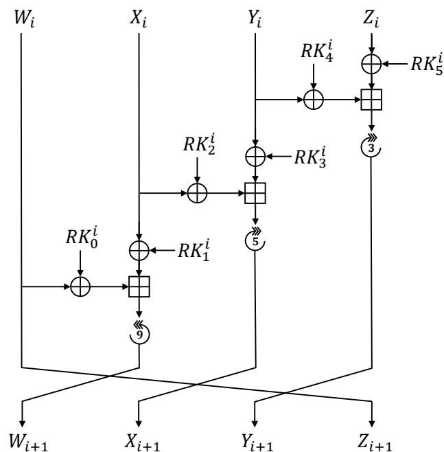
Figure 2. Round function of Lightweight Encryption Algorithm (LEA).
