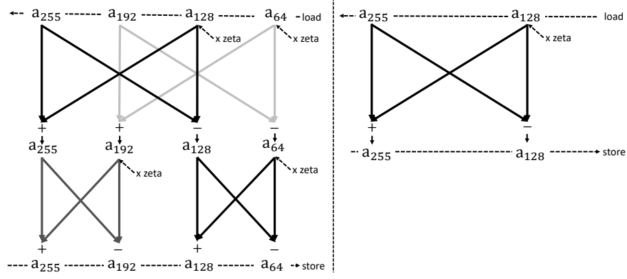
Fig. 2: Register scheduling for NTT
