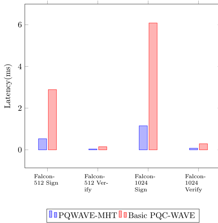
Fig. 2: PQWAVE-MHT and Basic PQC-WAVE Latency comparison
