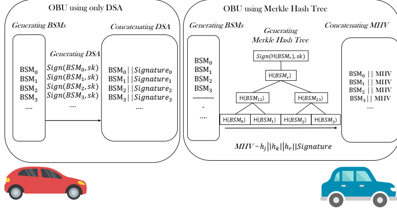
Fig. 1: Comparison of signature generation between the original case and our proposal using Merkle Hash Tree
