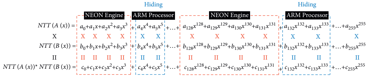
FIGURE 4: The proposed interleaving modular multiplication utilizing both the ARM processor and NEON engine.
