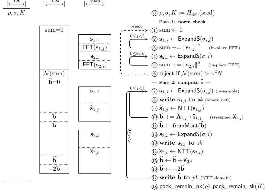
Figure 3: Streamed memory layout of HAETA5 key generation ( d=0 ). Two caller-level unions (1 024 B and 2 048 B) share memory across passes. Pass 1 checks the norm; Pass 2 computes \hat{\mathbf{b}} = \text{NTT}(-2\mathbf{b}) .
