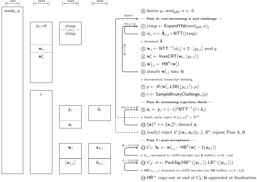
Figure 4: Streamed memory layout of pass-decomposed HAETAE signing. The driver keeps seeds and \mu (160 B) plus three 1024 B polynomial slots reused across passes. Dashed arrow: rejection loop (Pass A + B); Pass C runs once after acceptance. C_1/C_2 use reverse-order loops to stream directly to the rANS encoder.
