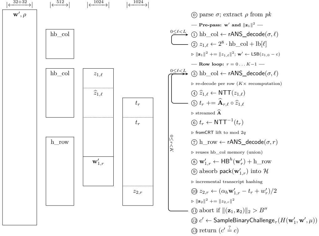
Figure 5: Streamed memory layout of row-streamed HAETAE verification. Four slots: persistent buffers (64 B), a 512 B union alternating high-bits columns and hint rows, and two 1024 B polynomial slots. Each row re-decodes HB^{z_1}(z_1) via streaming rANS, trading factor- k re-computation for eliminating a full polyveck buffer.
