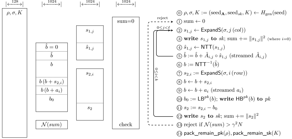
Figure 2: Streamed memory layout of HAETAE-2,3 key generation ( d > 0 ). Two polynomial slots (poly \mathbf{b} , \mathbf{s} ) and one norm accumulator ( \text{sum}[N] ) are reused across the streamed \hat{\mathbf{A}} expansion. Dashed arrow: rejection loop.
